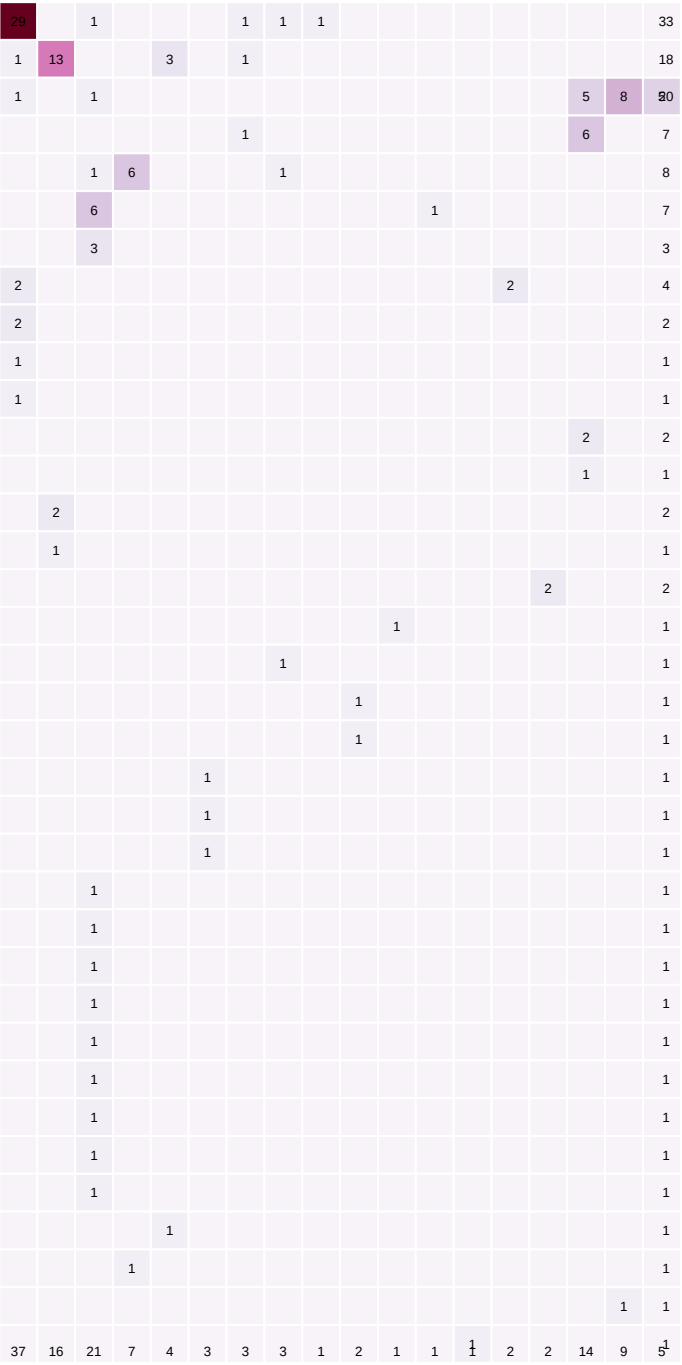
Reference groups – ARI = 0.49
